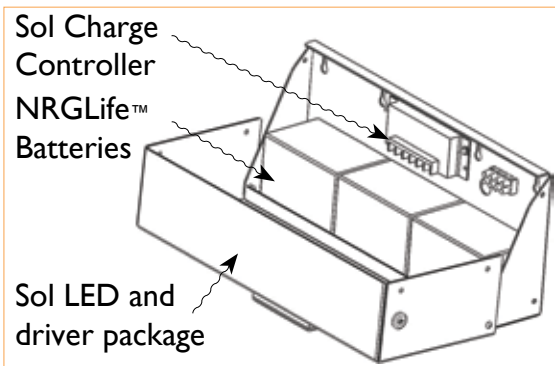
Self-contained low-profile shelter lighting package
