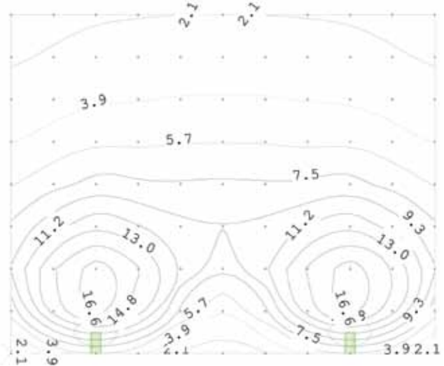
8 x 10 foot sign (2 fixtures) North view
