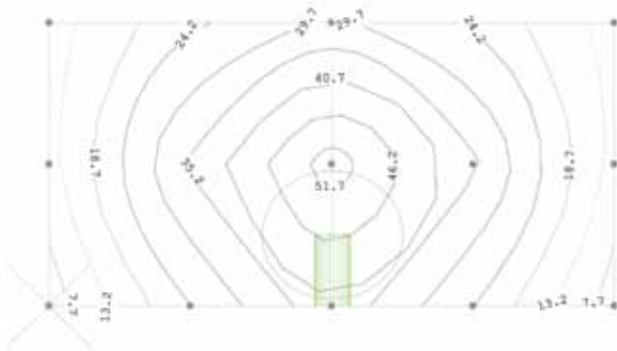
2 x 4 foot sign (1 fixture) North view
